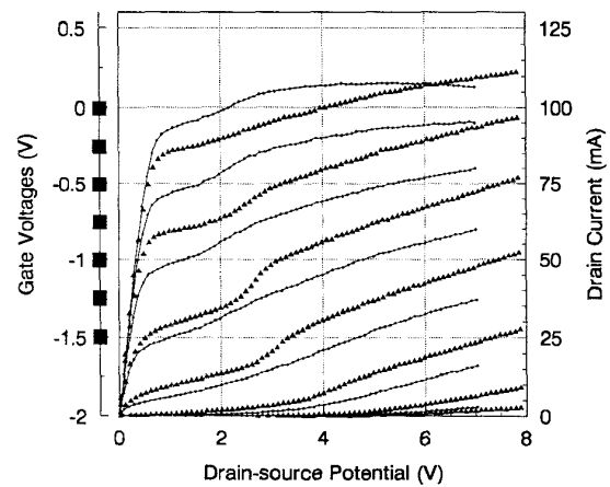
Fig. 7. Drain characteristics of the FET measured at 100C with 2\mu s pulses ( \Delta ) and at 20C with 10ms pulses ( \bullet ). Again the gate-voltage steps corresponding to the characteristic traces are plotted on the left-hand y -axis.
