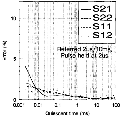
Fig. 4. Average discrepancy from 2–10GHz between S-parameters of the GaAs FET measured in 2\mu\text{s} pulses spaced 10ms and the S-parameters measured with a range of quiescent intervals but the same pulse interval of 2\mu\text{s} .
